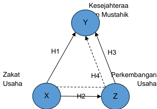
Figure 1. Model Penelitian
